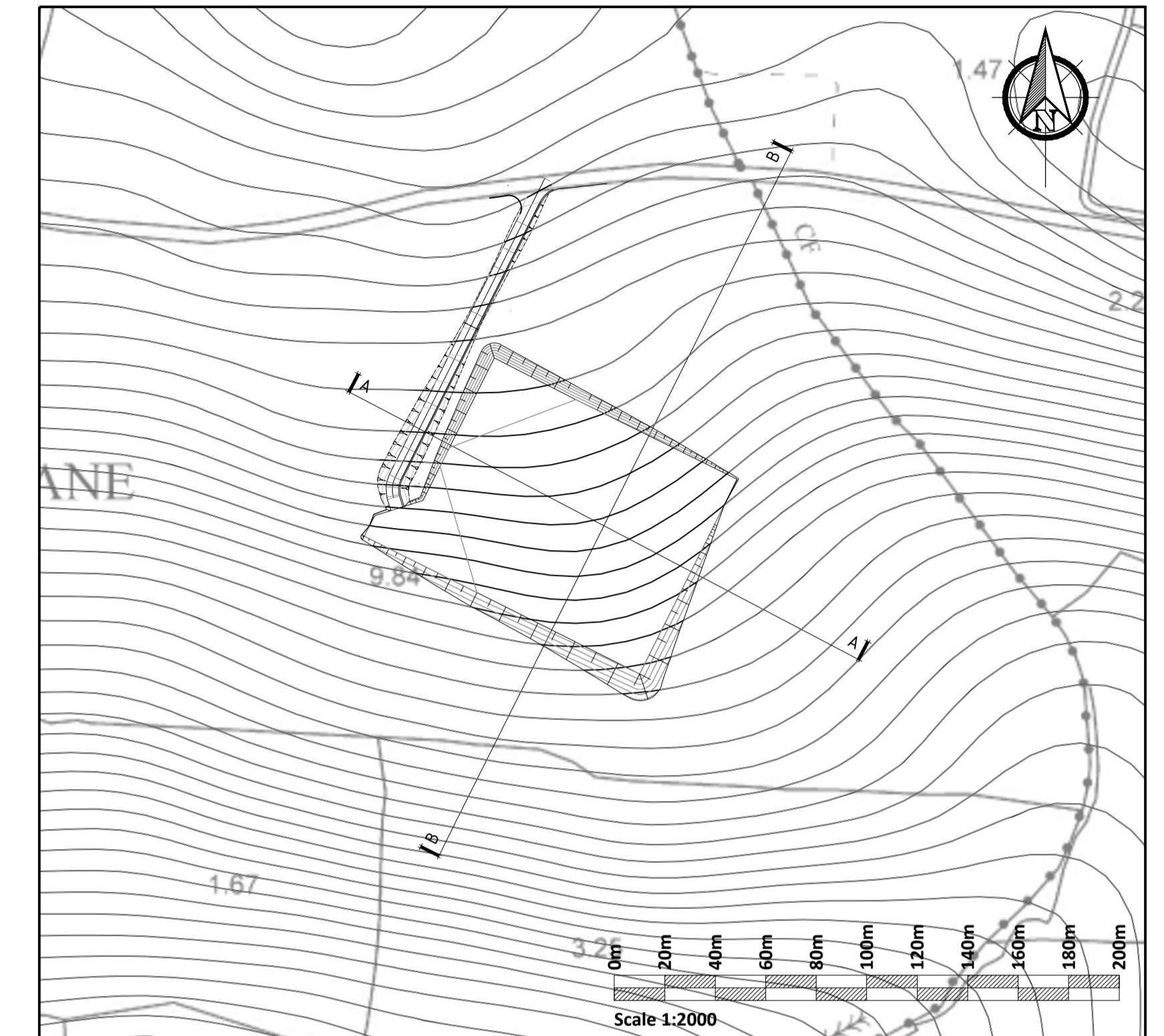
KEYPLAN Scale 1:2000
